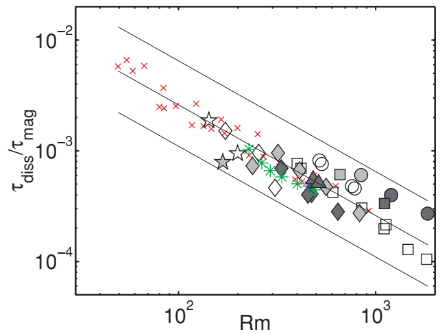
Figure 5. Magnetic dissipation time \tau_{\text{diss}} , normalized by the standard magnetic diffusion time \tau_{\text{mag}} , as a function of the magnetic Reynolds number Rm . Symbols as in Fig. 3, except the red crosses which represent the Christensen & Tilgner (2004) models. Our data set is filtered to exclude the non-dynamo run.
