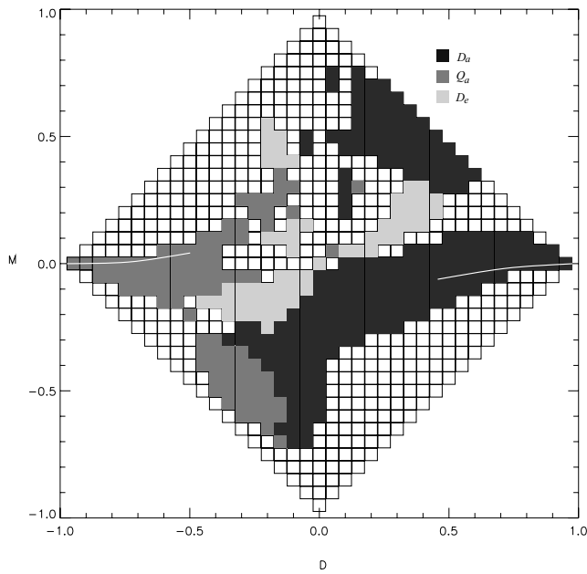
Figure 2. Dynamo action of two-parameter family of flows. Blank squares do not support dynamo action. Greyscale gives solution symmetry with lowest R_m^c . White lines are where oscillatory solutions have been found corresponding to oscillatory solutions in the Braginsky limit. After Gubbins & Gibbins (2002).
