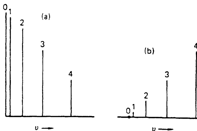
Figure 59 9 . - Patterns of Stark components for transitions in the rotation of an asymmetric top molecule. a) J = 4 \rightarrow 5 transition; b) J = 4 \rightarrow 4 transitions. The electric field is large enough for complete spectral resolution.
