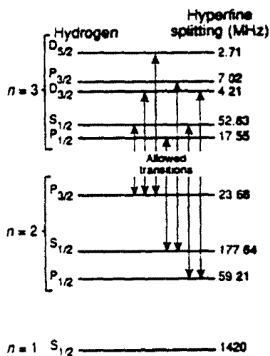
Figure 50. 6 Hyperfine structure in the n = 2 to n = 3 transition of hydrogen. The hyperfine splitting (MHz) are indicated at the right-hand side of each level.
