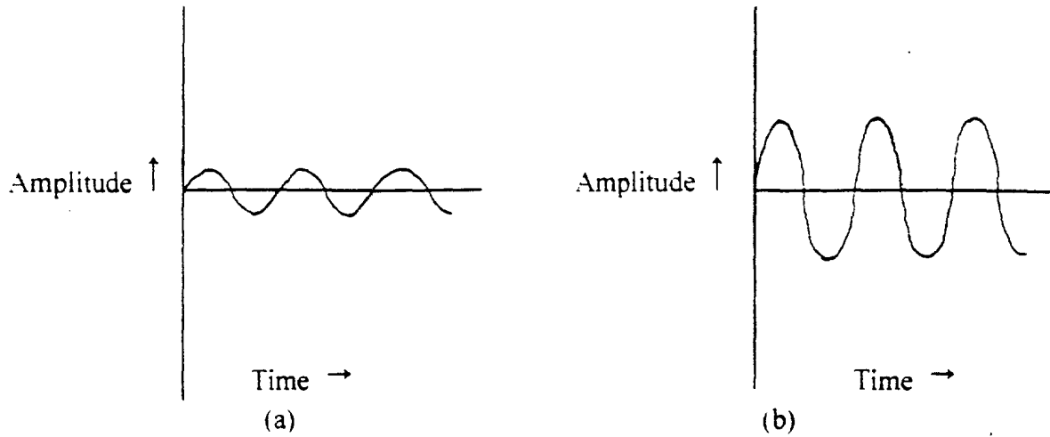
Figure 2. - Waves of different amplitudes but the same frequency. (a) Low intensity wave with low amplitude. (b) High intensity wave with high amplitude.
