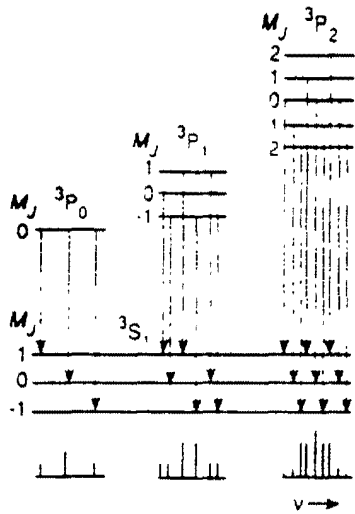
Figure 66 b - Anomalous Zeeman effect for zinc ^3P \rightarrow ^3S .
