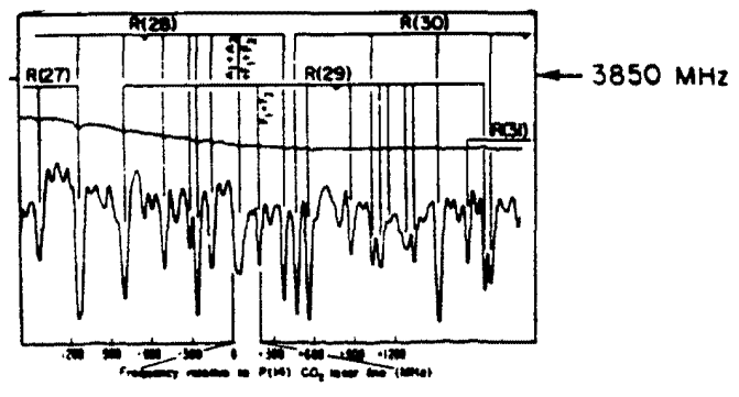
b) Fine structure frequencies shown in detail.
