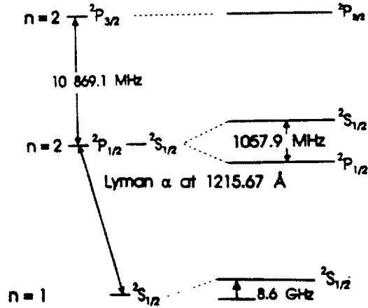
Figure 34. Fine structure of the n = 1 and n = 2 levels of the hydrogen atom. 19
