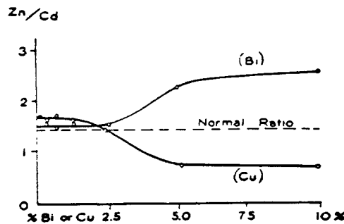
Figure 27 - Influence of copper and bismuth on the zinc/cadmium line ratio 10 .
