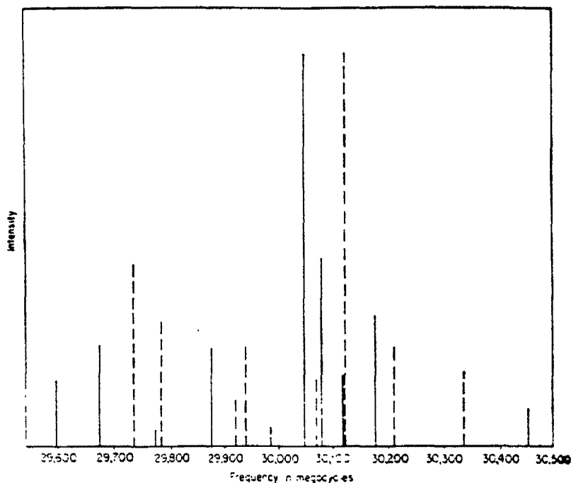
Figure 51. Hyperfine structure in the J = 1 → 2 rotational transition of CH 3 I.
