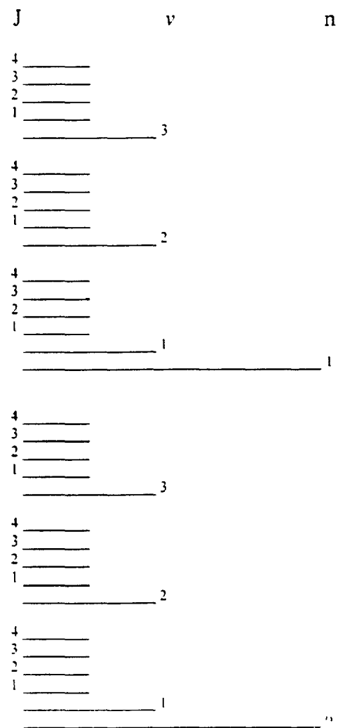
Figure 38. Diagram of rotational (J), vibrational (v), and electronic (n) energy levels for a molecule.
