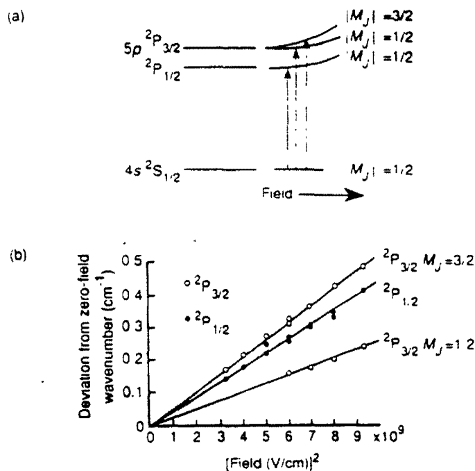
Figure 56 6 - The Stark effect for potassium. a) Schematic dependence of the 4s and 5p energy levels on the electric field. b) A graph plotting the deviation from zero-field positions of the 5p^2P_{1/2,3/2} \leftarrow 4s^2S_{1/2} transition wavenumbers against the square of the electric field.
