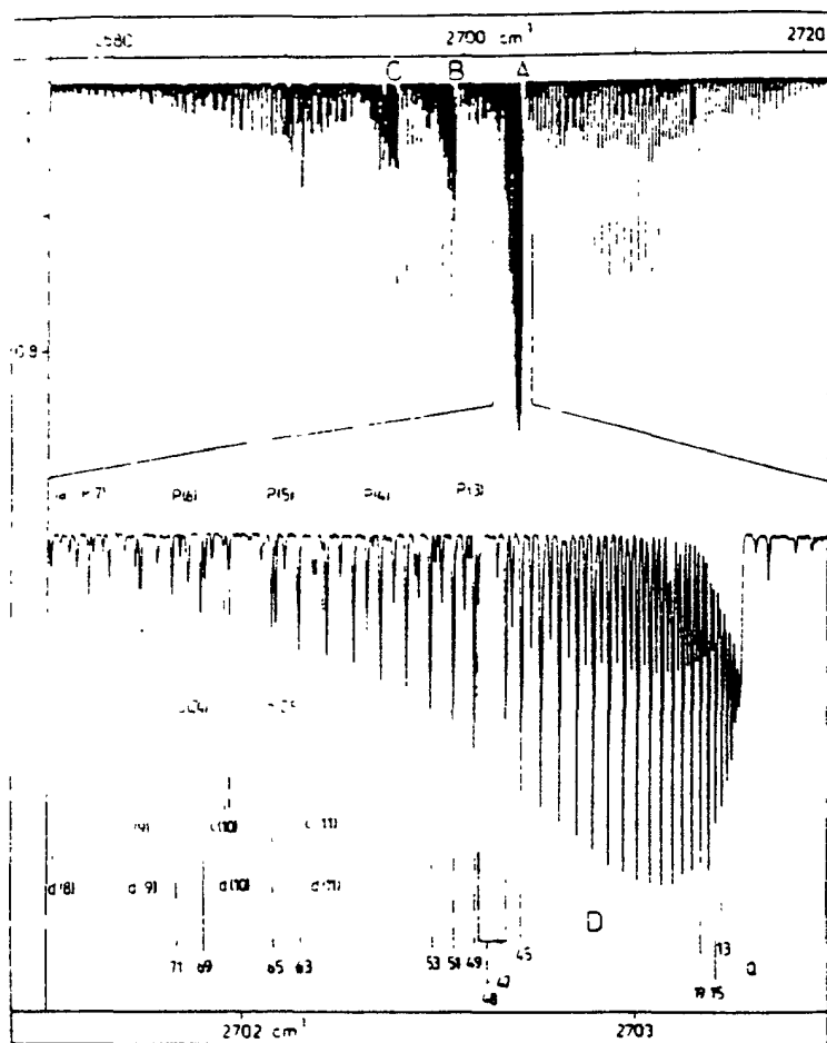
Figure 41. 21 The \nu_1 - \nu_3 band of FCCF. \nu_1 is vibrational level one, and \nu_3 is vibrational level 5. The vibrational level frequencies heterodyne (add and subtract) just like all frequencies. The additive heterodyne of \nu_1 and \nu_3 are depicted in the spectral band showing the frequency band at "A" ( \nu_1 + \nu_3 ). B = \nu_1 - 2\nu_3 .
