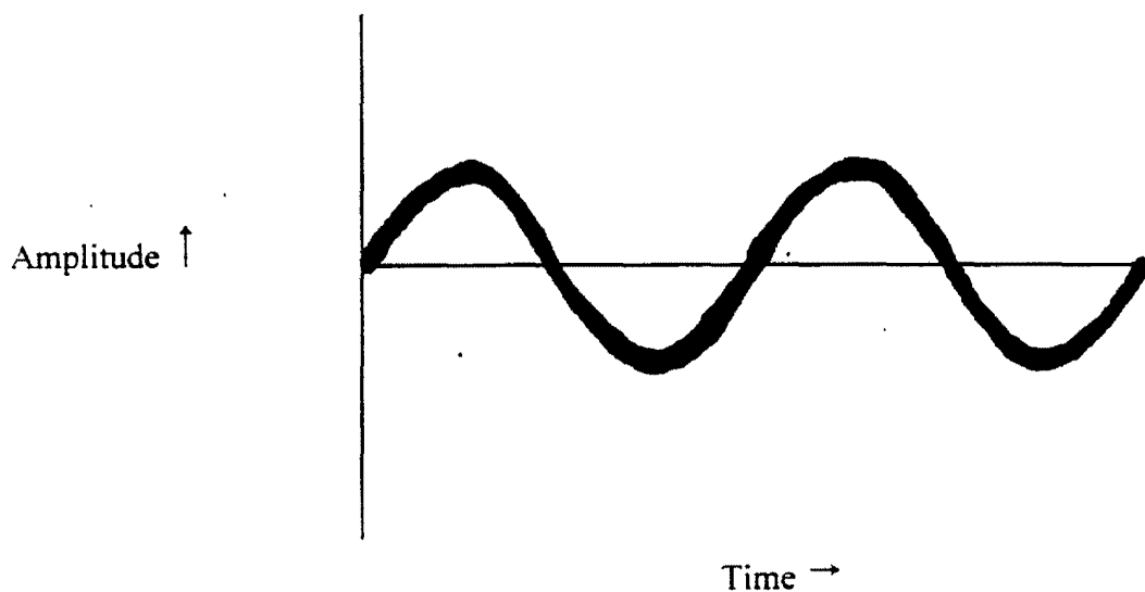
Figure 1. - Wave representation (acoustic or electromagnetic)
