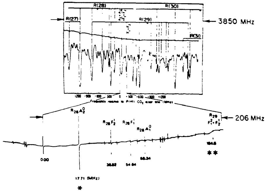
Figure 48. SF 6 fine structure spectrum with a small portion from zero to 300 magnified. 2
