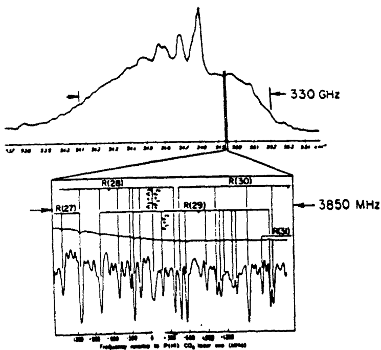
Figure 47. SF 6 rotation-vibration band and fine structure frequencies. 2
