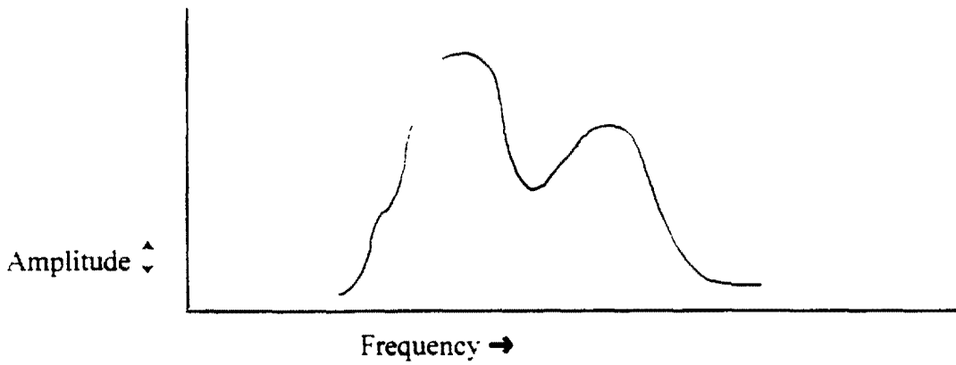
c) Spectral pattern at high temperature.
