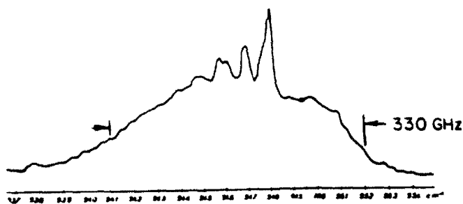
Figure 36. The vibration band of SF 6 at wavelength 10 μm. 2
