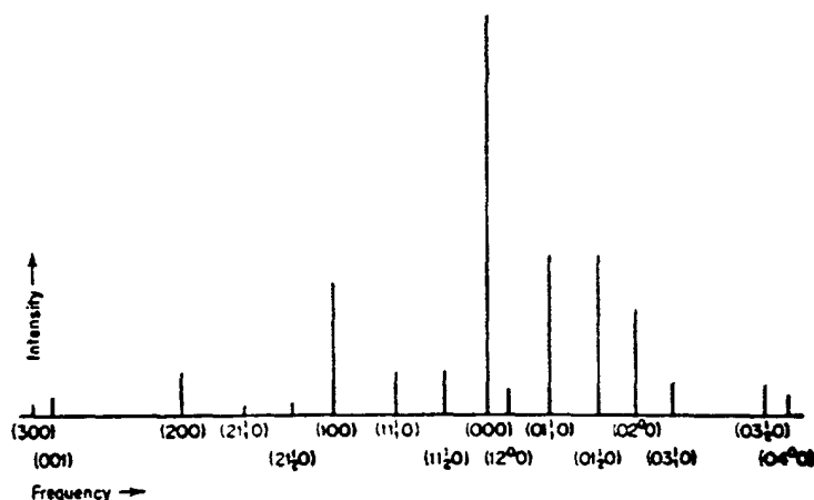
Figure 46. 9 Rotational transition J = 1 \rightarrow 2 for the triatomic molecule OCS. The vibrational state is given by vibrational quantum numbers in brackets (v_1, v_2, v_3) , v_2 having a superscript |l| . In case l = 1 , a subscript 1 is applied to the lower-frequency component of the l -type doublet, and 2 to the higher-frequency component. The two lines at (01 1 0) and (01 2 0) are an l -type doublet, separated by q_l .
