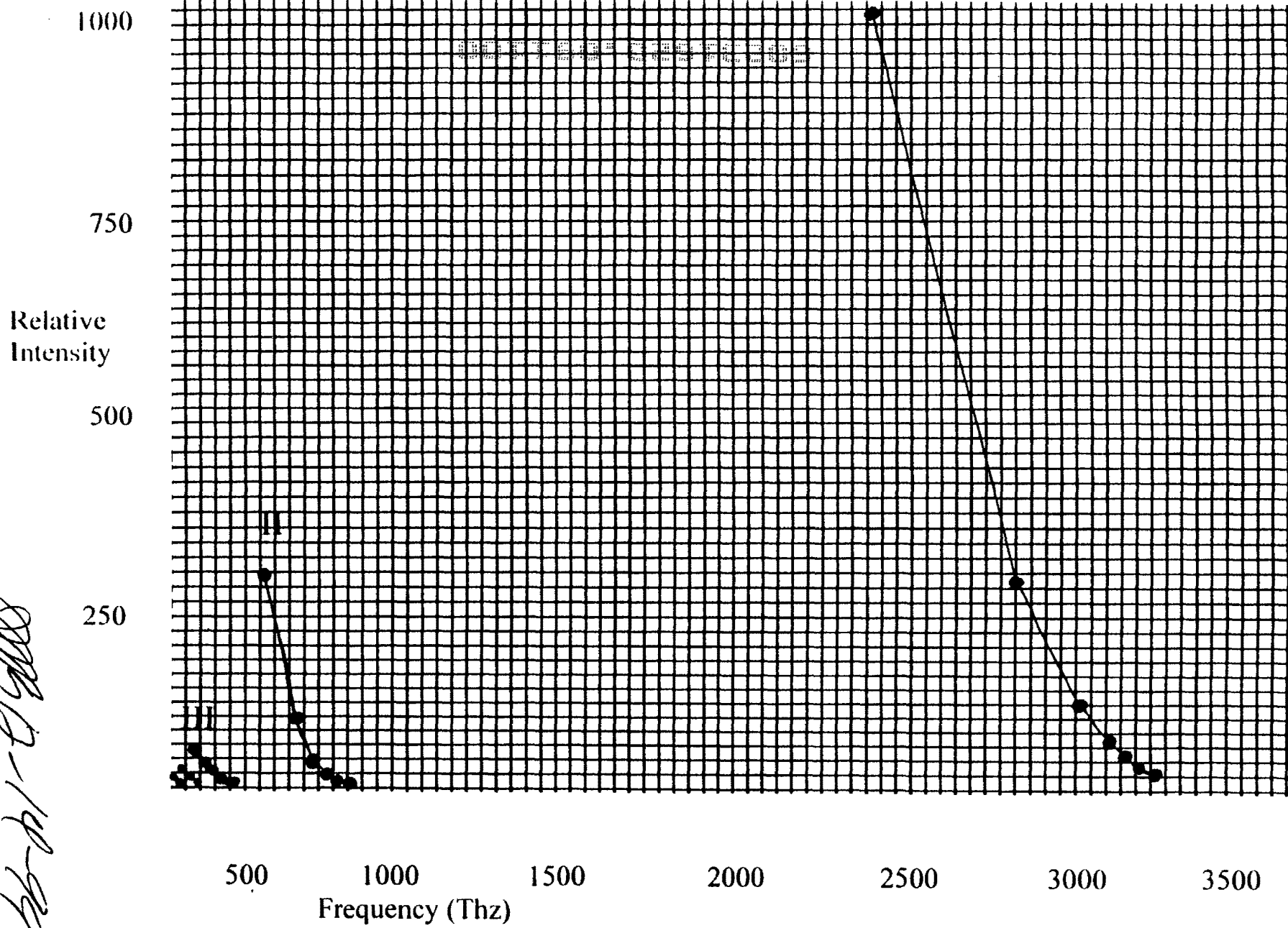
Figure 8. - Frequency diagram of hydrogen
