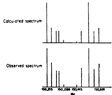
Figure 53. 9 - Energy level diagram and hyperfine frequencies for the NO molecule.
