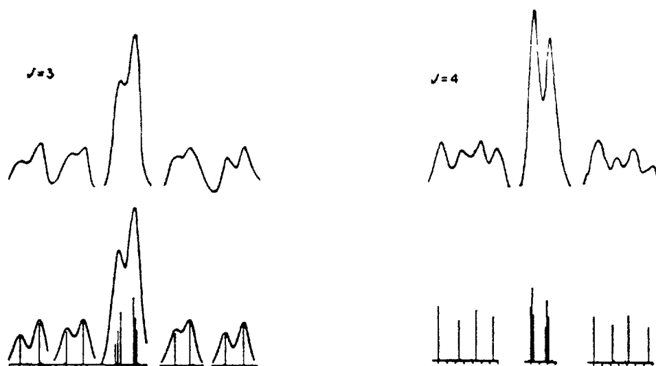
Figure 55. 9 - Hyperfine structure and doubling of the NH 3 spectrum for rotational levels J = 3 and J = 4. The upper curves show experimental data, while the lower curves are derived from theoretical calculations. Frequency increases from left to right in 60 KHz intervals.
