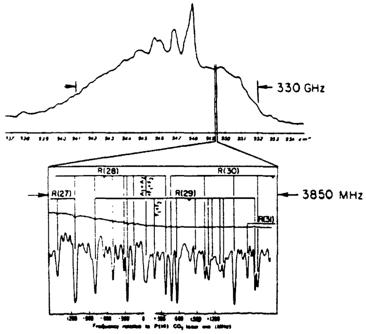
a) Slice from vibration band of SF 6 .
