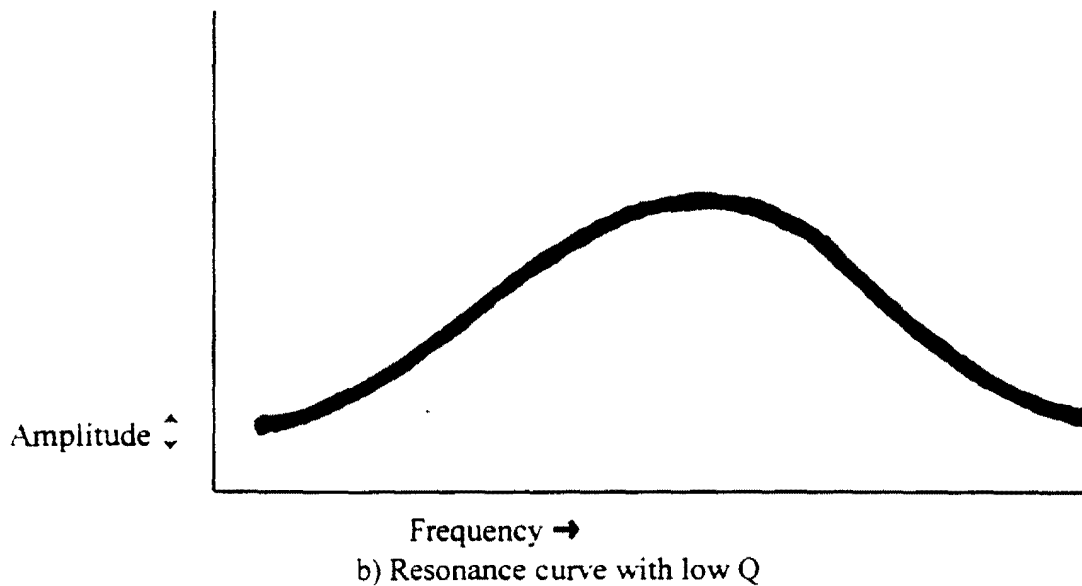
Figure 13. Resonance curves with different resonance quality factors, Q. a) Narrow resonance curve with high Q; b) Broad resonance curve with low Q. ( Q = f_0 / (f_2 - f_1) )
