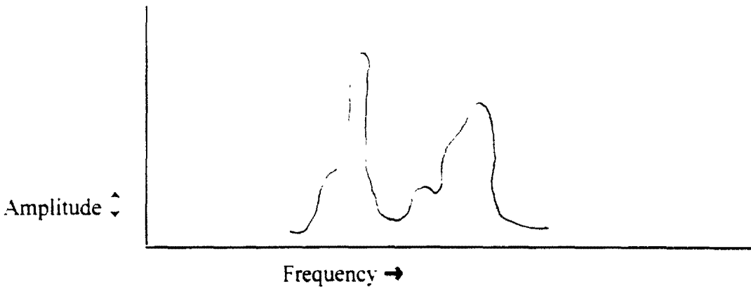
b) Spectral pattern at moderate temperature.
