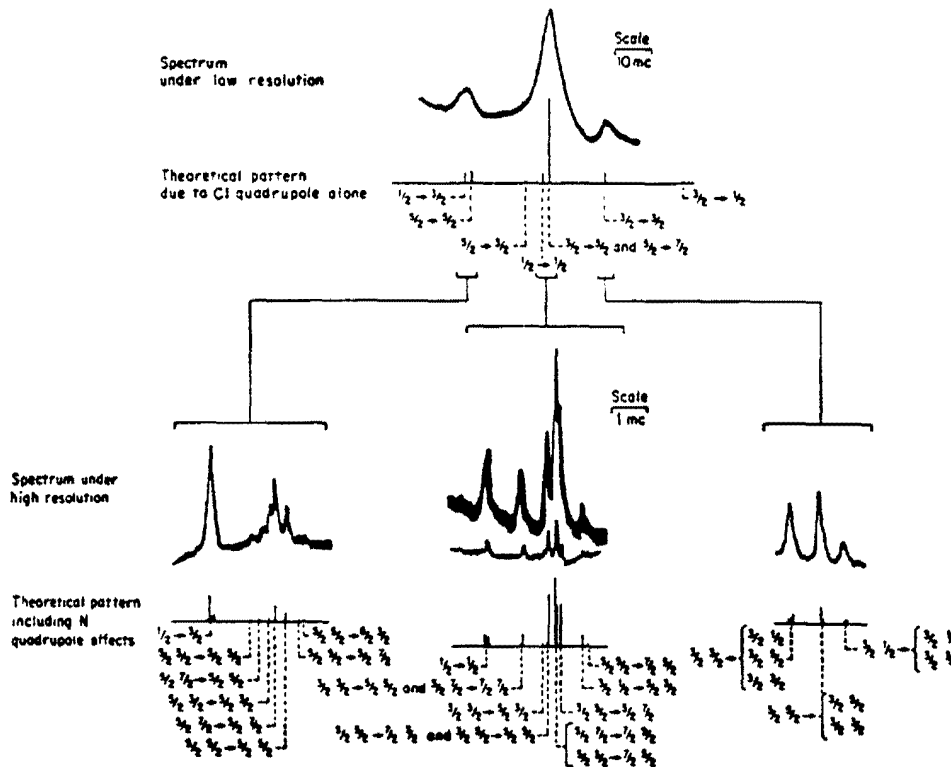
Figure 52. 9 - Hyperfine structure of the J = 1 \rightarrow 2 transition for C1CN in the ground vibrational state. Experimental values are compared to theoretical patterns.
