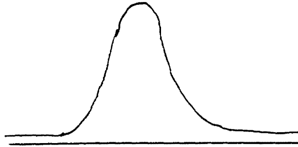
a) Normal spectral curve produced by a single atom
