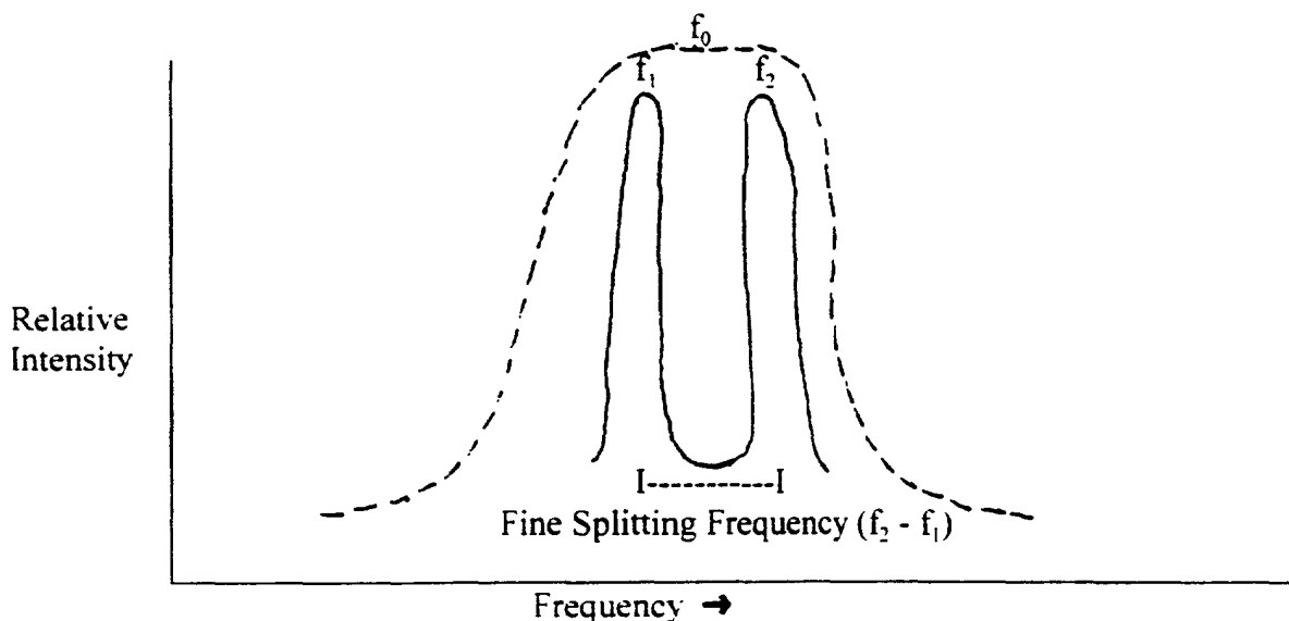
Figure 31. Fine structure. Dotted line (---) is electronic spectrum frequency. f_0 : solid lines (___) are fine structure frequencies. f_1 and f_2 . The difference (heterodyne) between the fine structure frequencies ( f_2 - f_1 ) is the fine splitting frequency.
