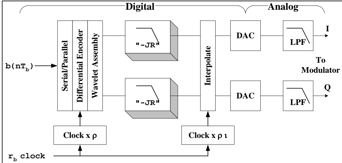
Figure 2-1. FQPSK-JR Baseband Signal Generator
