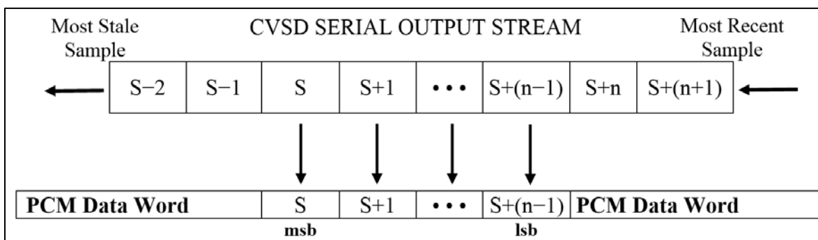
Figure 5-1. Insertion of CVSD-Encoded Audio into a PCM Stream
