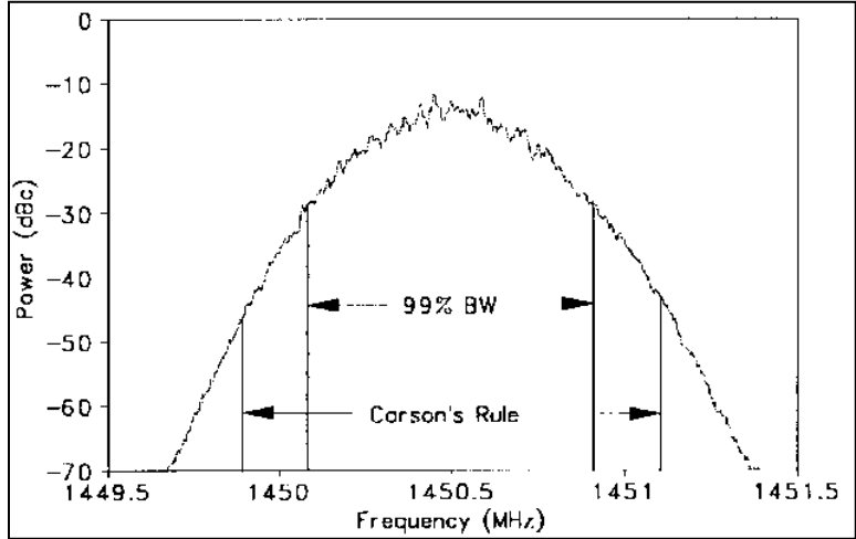
Figure A-7. FM/AM Signal and Carson's Rule
