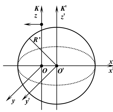
Fig.2 Image 2 of invariable speed of light.
