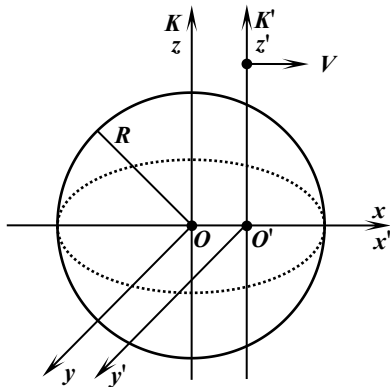
Fig.1 Image 1 of invariable speed of light.
