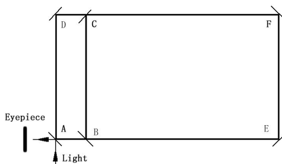
Fig.11 The schematic picture of the M-G experiment.
