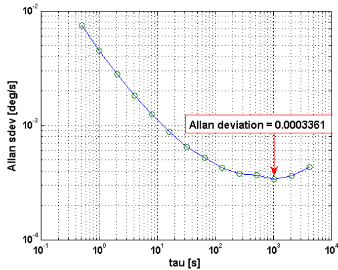
Figure 3: Allan deviation of SCC1300-D02 gyroscope
