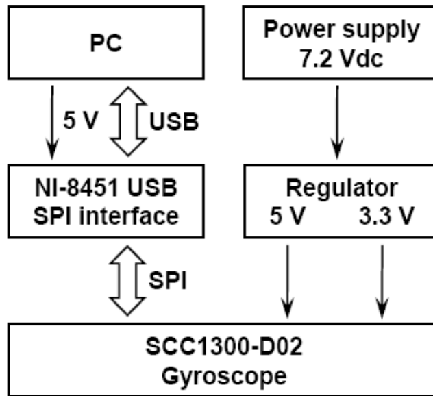
Figure 1: Block diagram showing the connections between the main components
