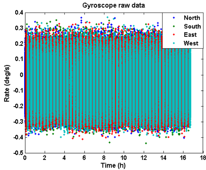
Figure 9: Raw data used for measuring the Earth's rotation rate
