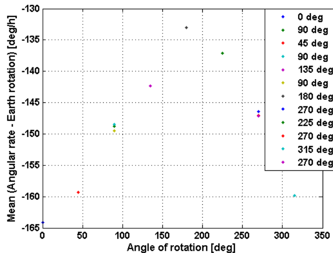
Figure 5: Average of the angular rate data without the Earth rotation
