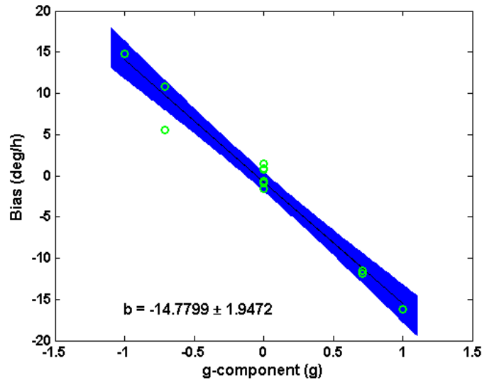
Figure 6: Linear least squares of the g-sensitivity
