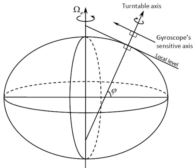
Figure 7: The sensitive axis of the gyroscope is perpendicular to the local vertical while the turntable rotates
