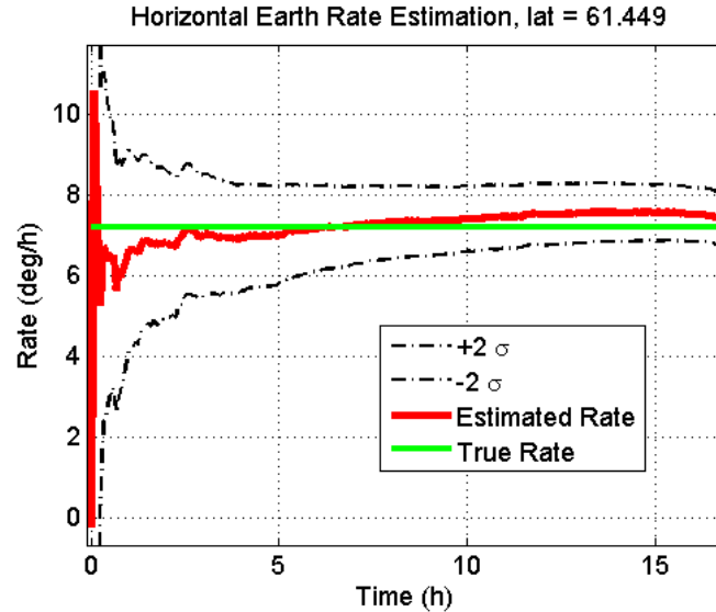
Figure 11: Kalman filter output
