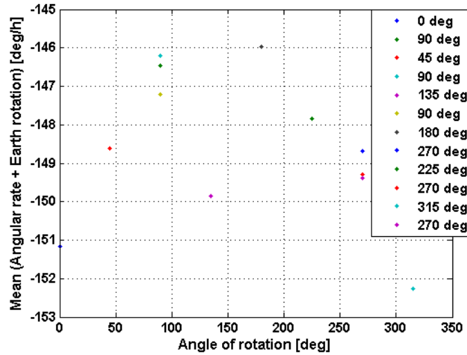
Figure 4: Average of the angular rate data
