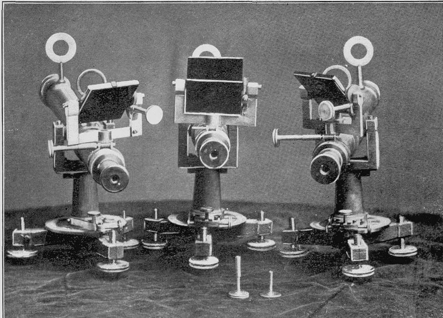
HELIOPTOPES OF LATEST PATTERN.
