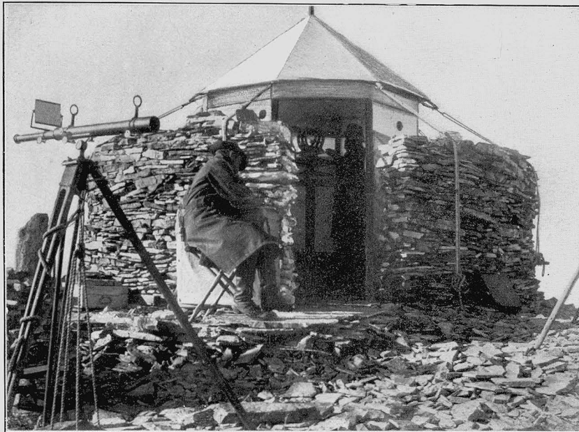
HIGH SUMMIT STATION, TUSHAR MOUNTAIN, UTAH, SHOWING RING WALL AND DOUBLE SHELTER TENT AGAINST STORMS AND RADIATION OF HEAT.
