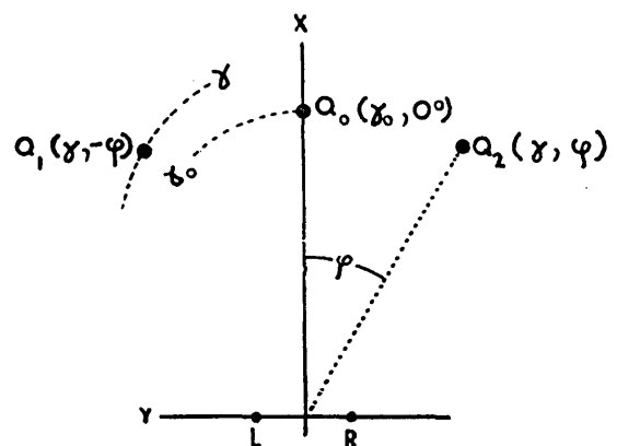
FIG. 4. Experimental situation in Helmholtz's three-rod experiment. Q(\gamma, \pm\varphi) are the fixed lights; Q_0(\gamma_0, 0^\circ) is the light movable along x -axis.
