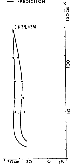
FIG. 14. The broad alley experiment with Observer W.K.; Values of constants observed in the 3 and 4 point tests: \sigma=16.9 , K=-0.55 ; Values of constants observed in the alley experiment: \sigma=17.8 , K=-0.57 .
