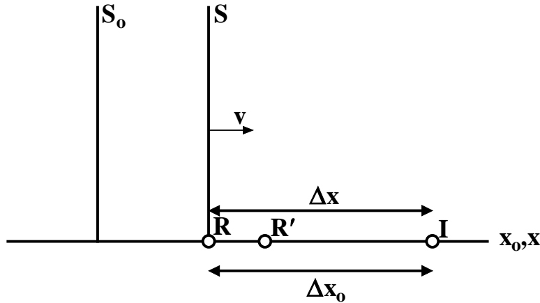
Fig.1 Inertial Frames in Relative Motion at time t_o = T_o
