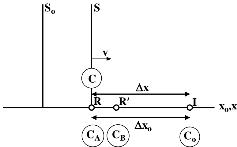
Fig.2 Synchronized clocks C_A , C_B and C_o in S_o and clock C in S at time t_o = T_o
