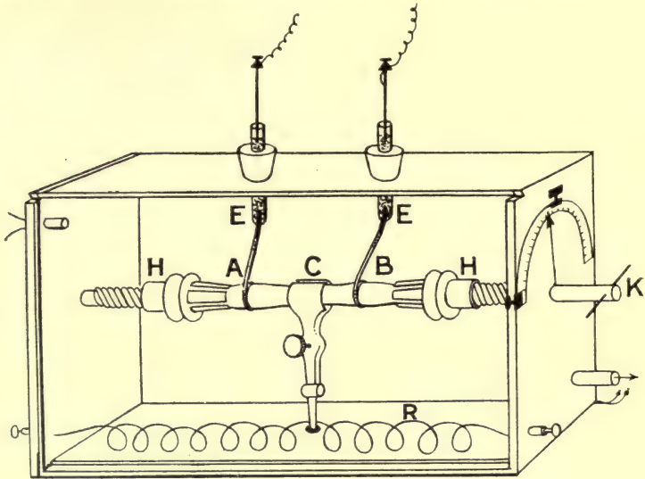
FIG. 37.—THE GLASS CHAMBER CONTAINING THE PLANT
