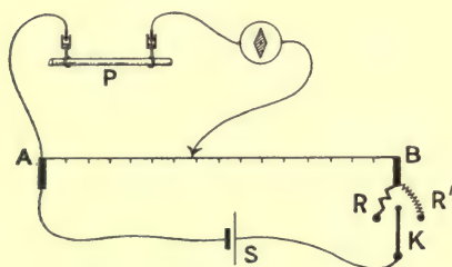
FIG. 9.—THE COMPENSATOR
