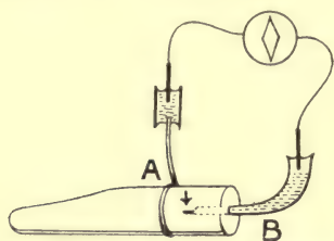
FIG. 29.—RADIAL E.M. VARIATION
