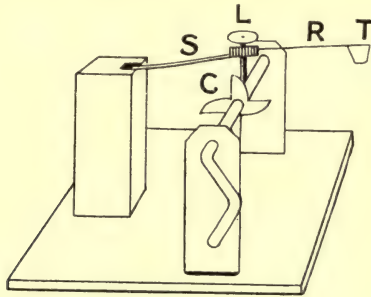
FIG. 10.—THE SPRING-TAPPER
