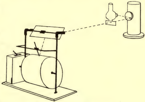
FIG. 8.—RESPONSE RECORDER
