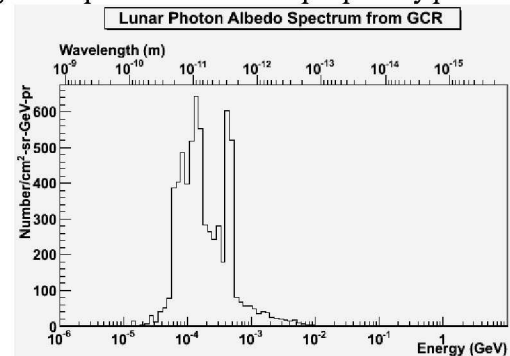
Figure 1: Photon luminescence of the Moon [1].
